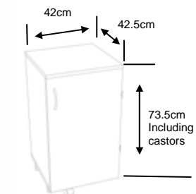
CLOSED - WIDE 42cm (16 1/2") DEEP 42.5cm (16 3/4") HIGH 73.5cm (29")
